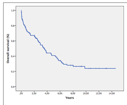
Figure 2. Kaplan-Meier global survival curves.
