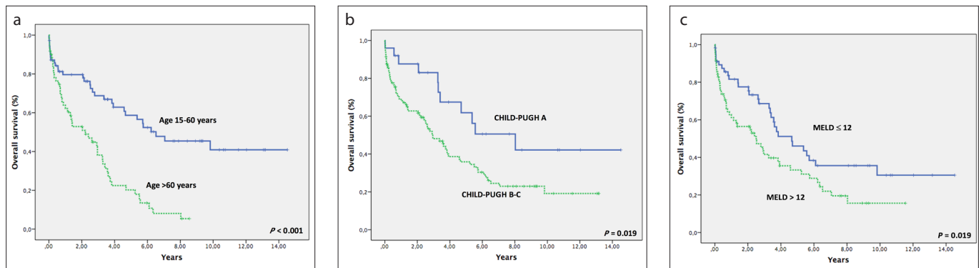
Figure 3. a–c. Kaplan-Meier curves of overall survival grouped by age (a), Child-Pugh (b) and MELD (c).
